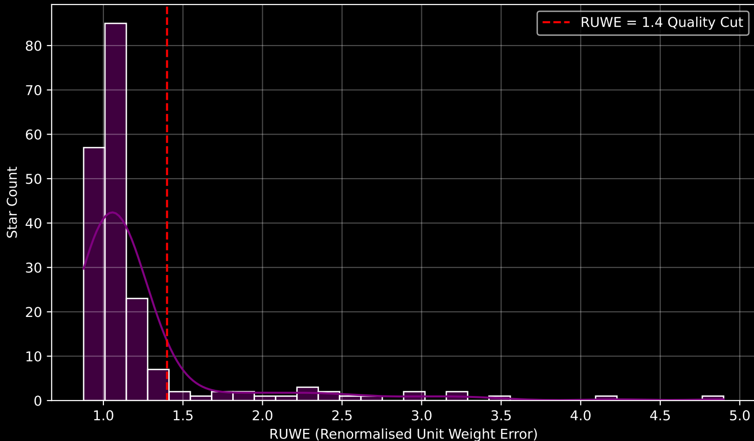
GAPOGEE DR17 Field [K2_C8_134-63] RUWE Distribution (n= 195)
