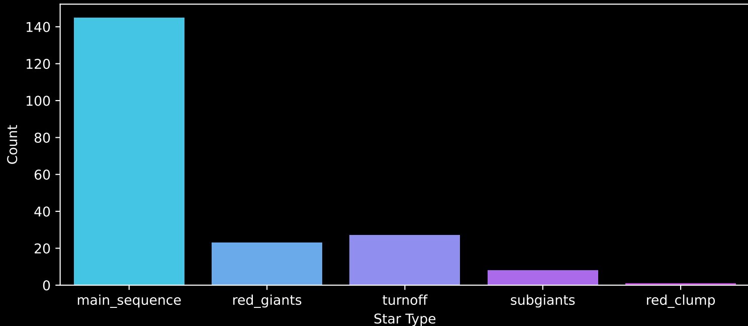
APOGEE DR17 Field: [K2_C8_134-63] Count plot of Star Type
