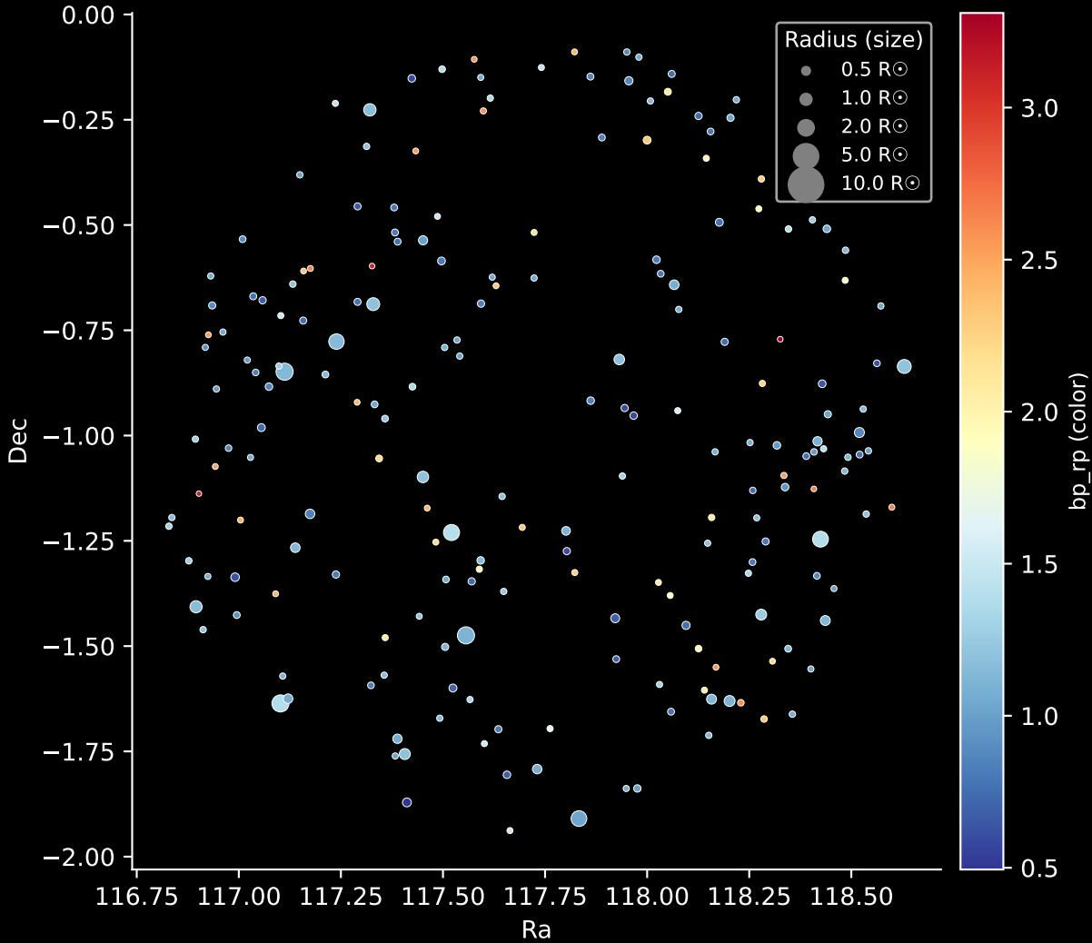
APOGEE DR17 Field: [K2_C8_134-63] Stars: 204
