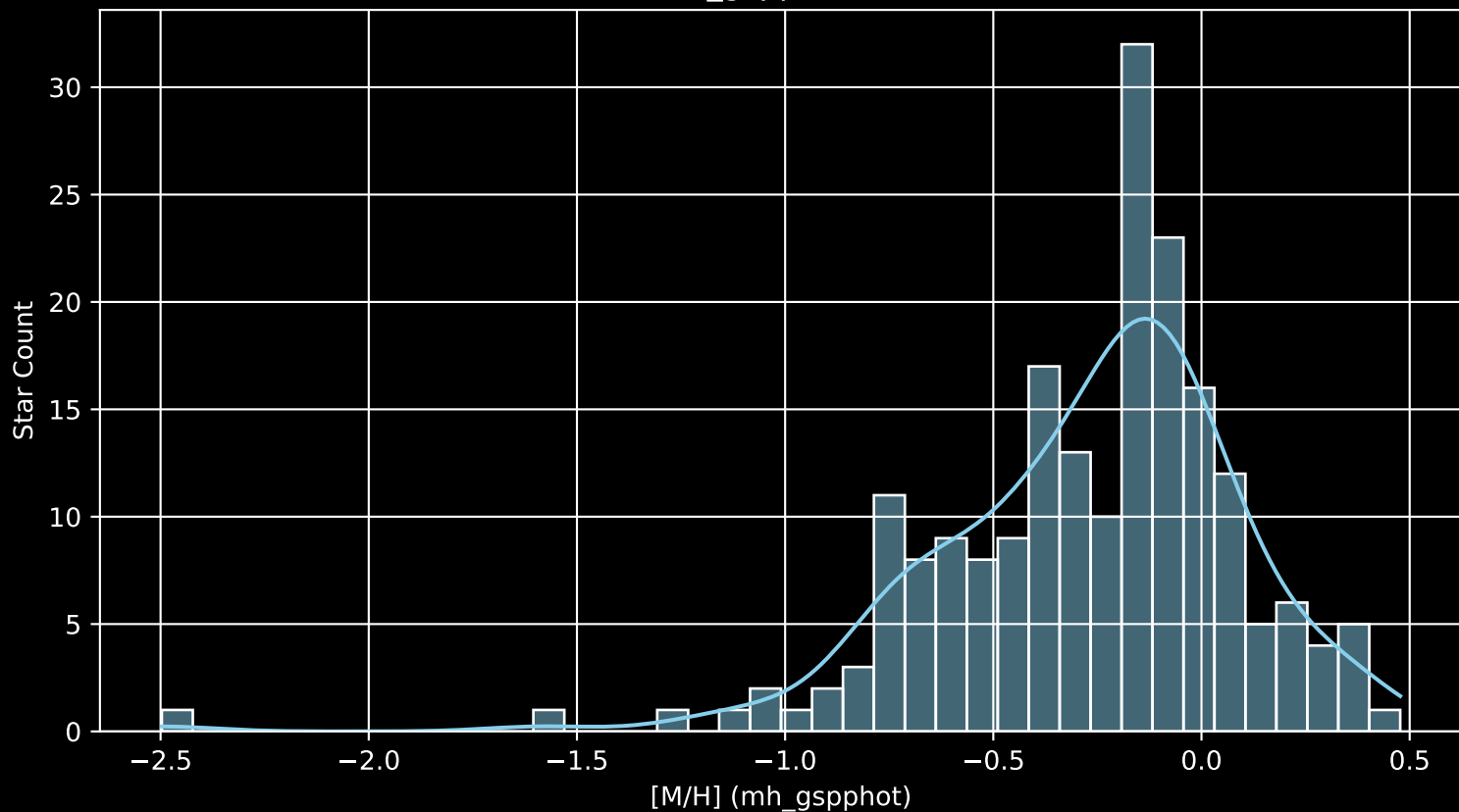
APOGEE DR17 Field: [K2_C8_134-63 [M/H] (mh_gspphot) (n= 201)
