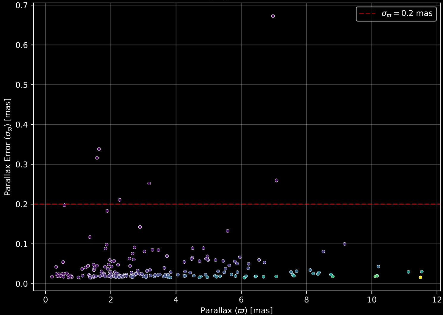
APOGEE DR17 Field: [K2_C8_134-63] Parallax Quality (n= 204)
