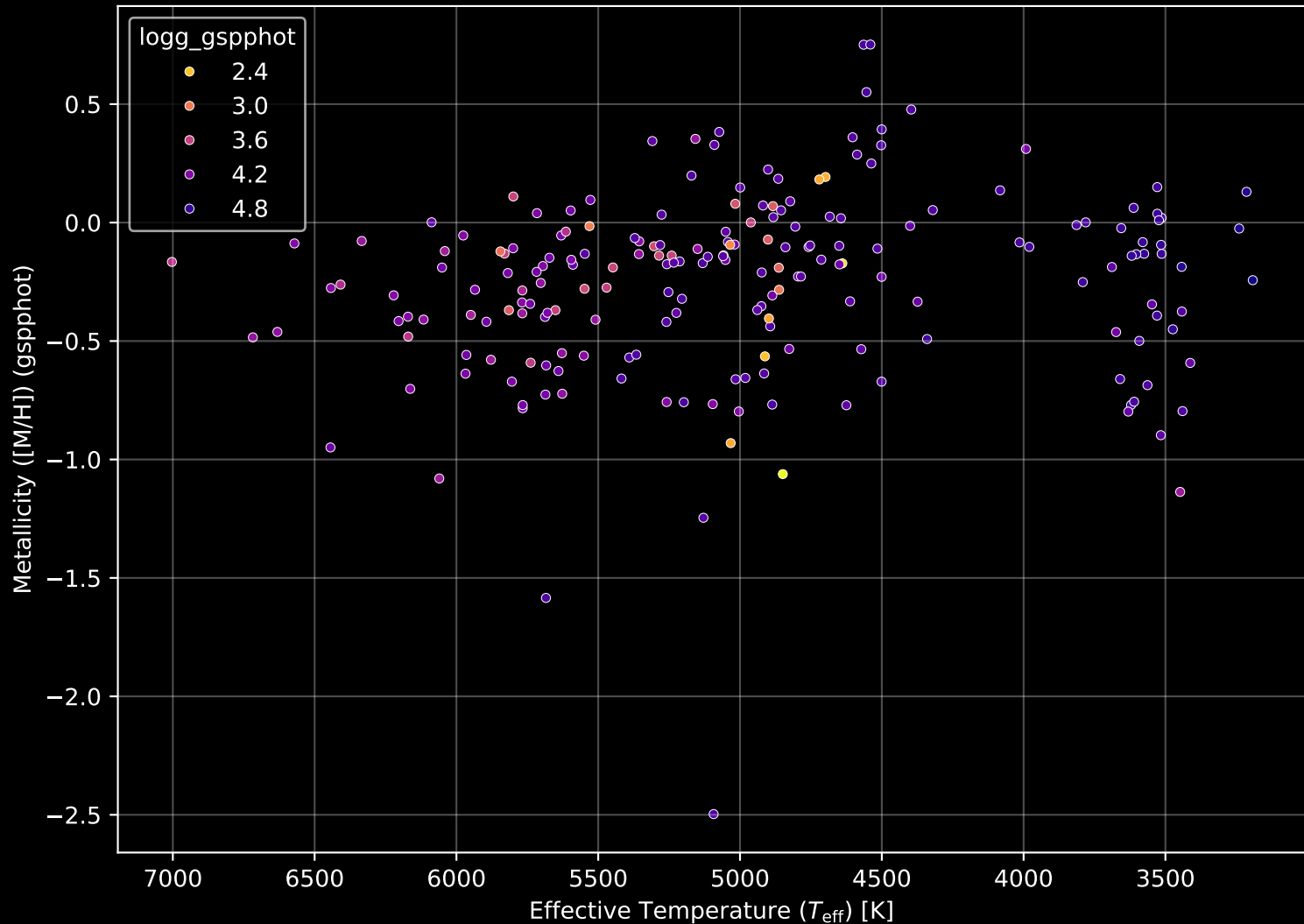
APOGEE DR17 Field: [K2_C8_134-63] Stellar Population Parameters (n= 204)
