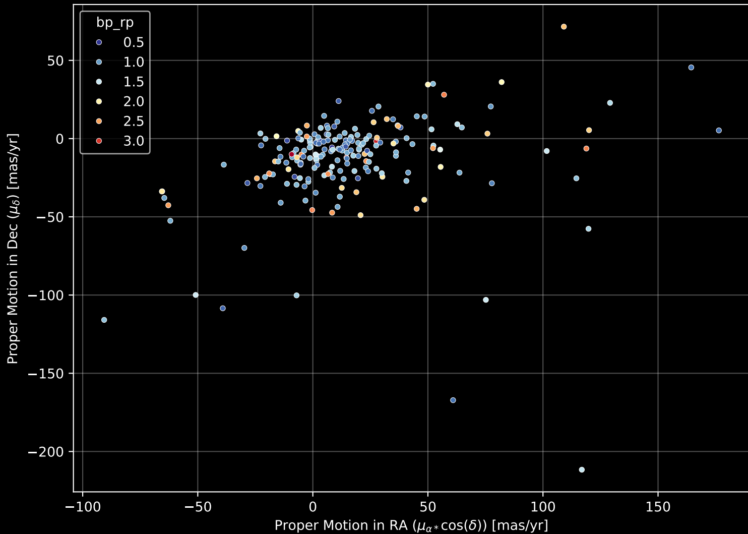
APOGEE DR17 Field: [K2_C8_134-63] Proper Motion Diagram (n= 204)
